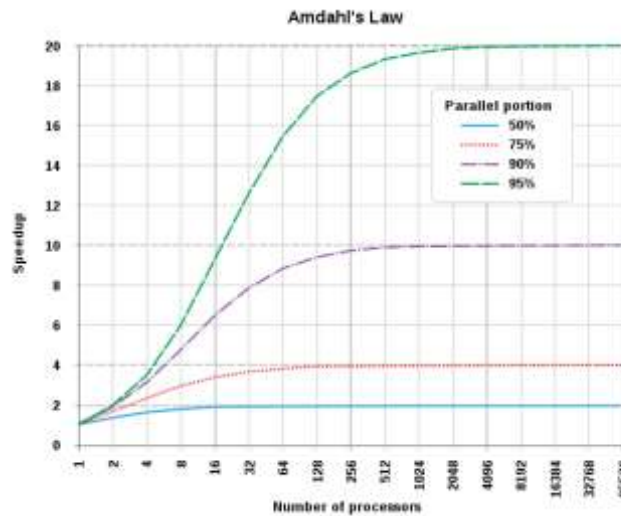
Figure 5: Graph Representation
